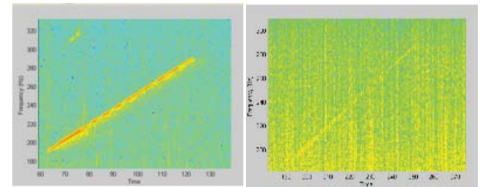
Source sweep recorded at the source location (left) and the sweep recorded 60 km west from the source (right).
