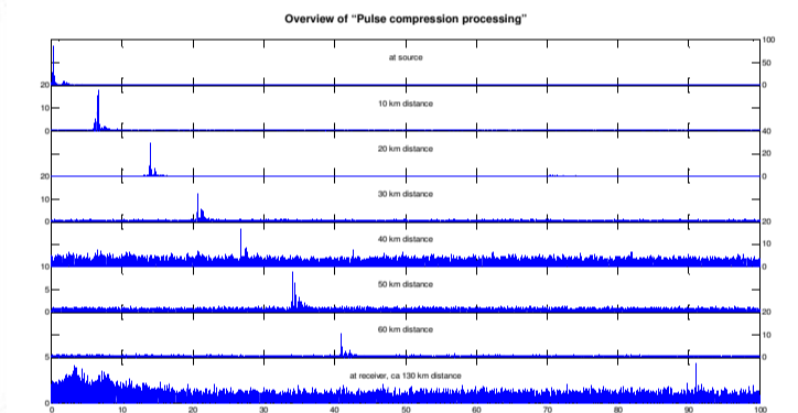
Figure 1: Overview of pulse compression processing for the tests in the line between source and receiver. The x-axis shows elapsed time since start of transmission. The y-axis is the crosscorrelation (unnormalized) between the received signal and the replica (190 to 290 Hz linear FM sweep in 60 seconds).
